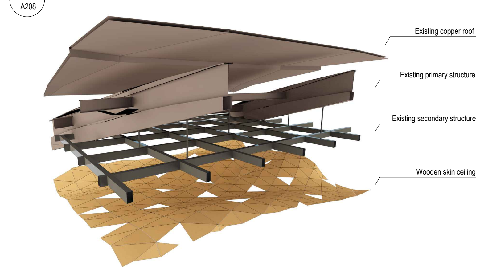
2 Roof Scheme
