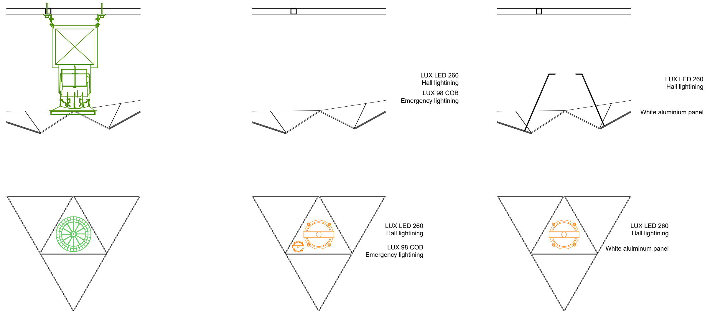
7 Ceiling Elements - Section
