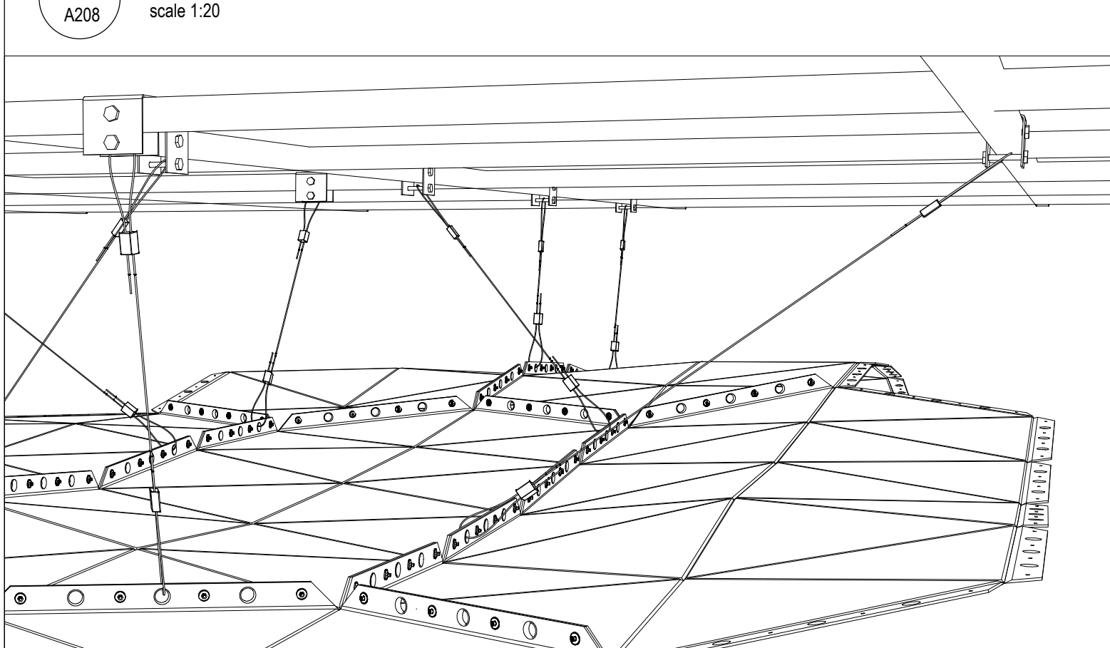
9 Ceiling Elements - 3d view
