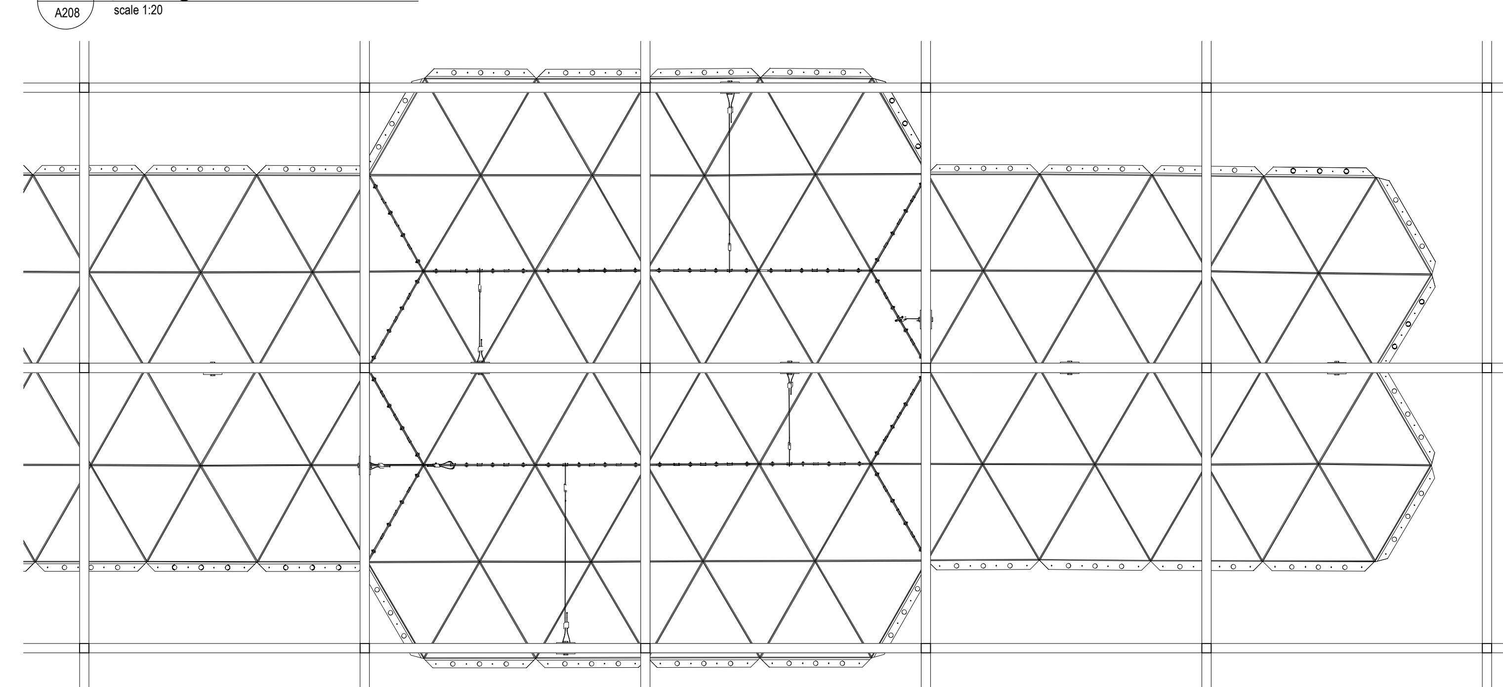
10 Ceiling Elements - Assembling
